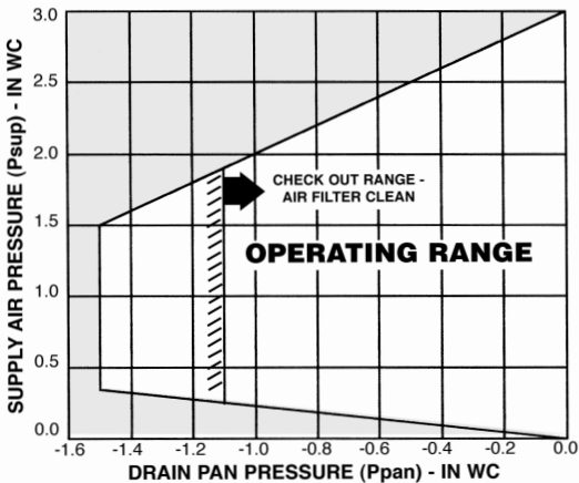
CostGard™ CONDENSATE DRAIN SEAL MODEL 1525-17-56 OPERATING RANGE
